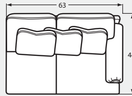
#31 RAF LOVESEAT 63Wx44Dx40H 1- 22" A Pillow 2- 22" B Pillow
