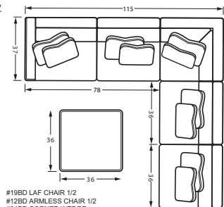
#19BD LAF CHAIR 1/2 #12BD ARMLESS CHAIR 1/2 #34BD CORNER WEDGE #12BD ARMLESS CHAIR 1/2 #18BD LAF CHAIR 1/2
